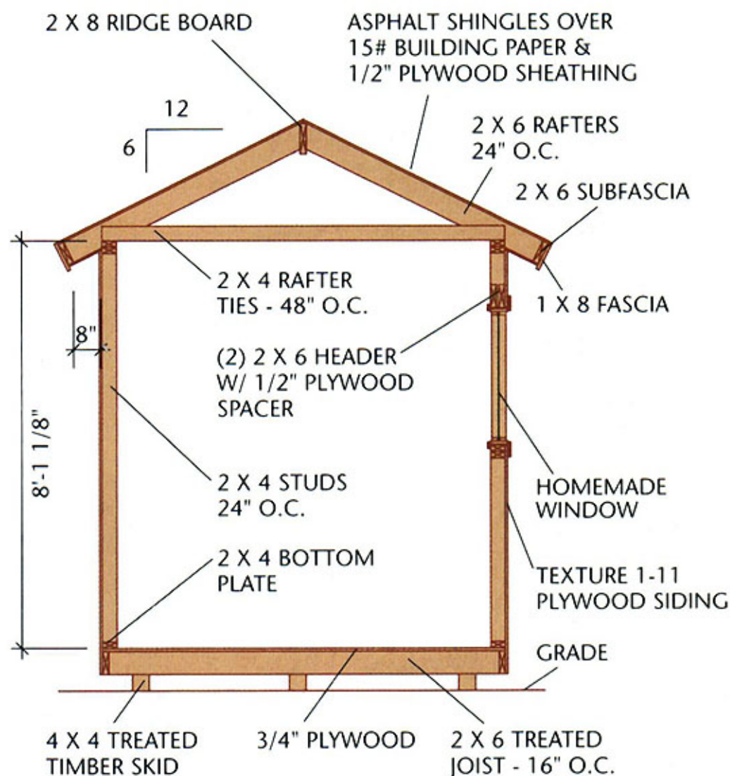
BUILDING SECTION
