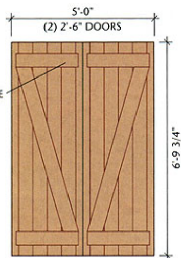
INSIDE ELEVATION
